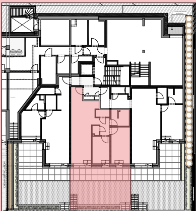
PLAN GENERAL - Rez-de-jardin
