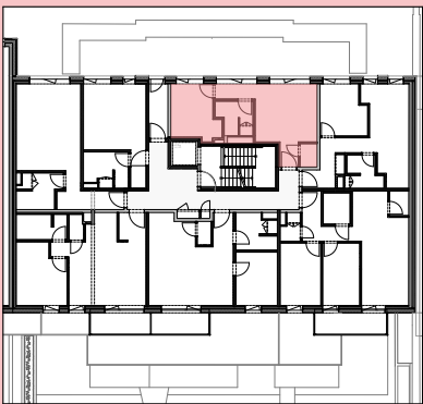
PLAN GENERAL - Rez +4
