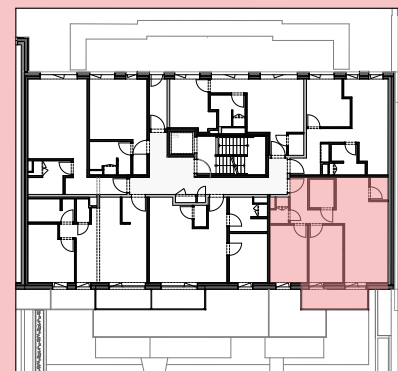
PLAN GENERAL - Rez +4
